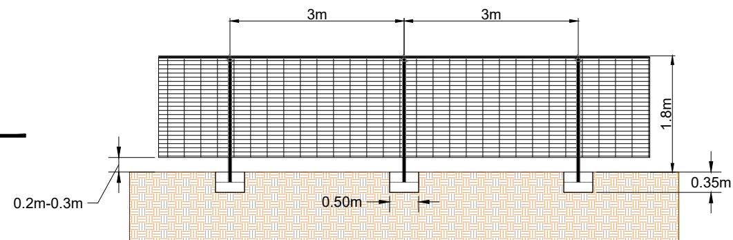
Fence: Front View
