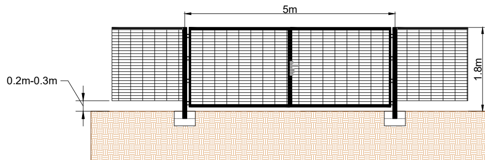
Regular doors in fence: Front View
