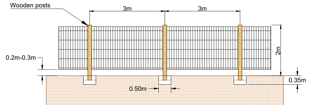
Fence: Front View
